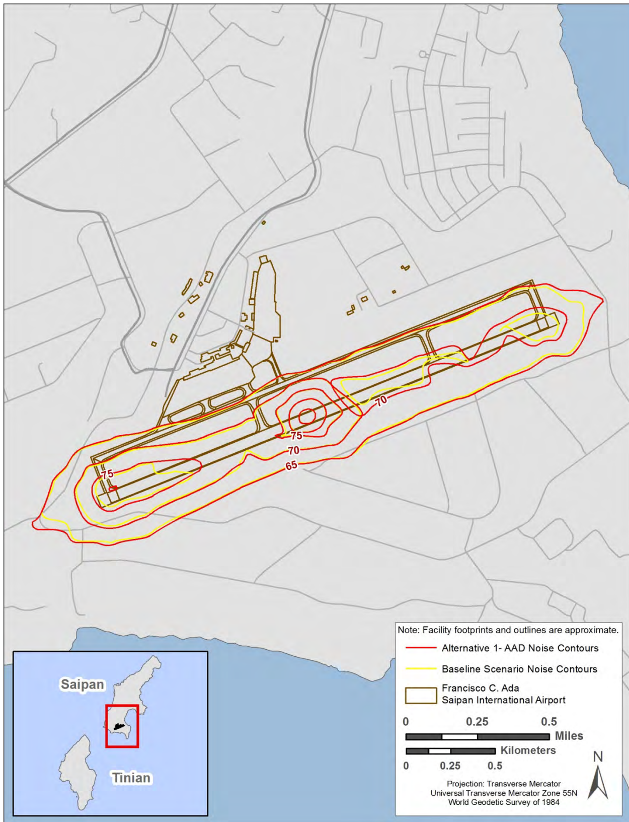
2 Figure 4.1-1. Alternative 1–AAD Noise Contours at Saipan International Airport
