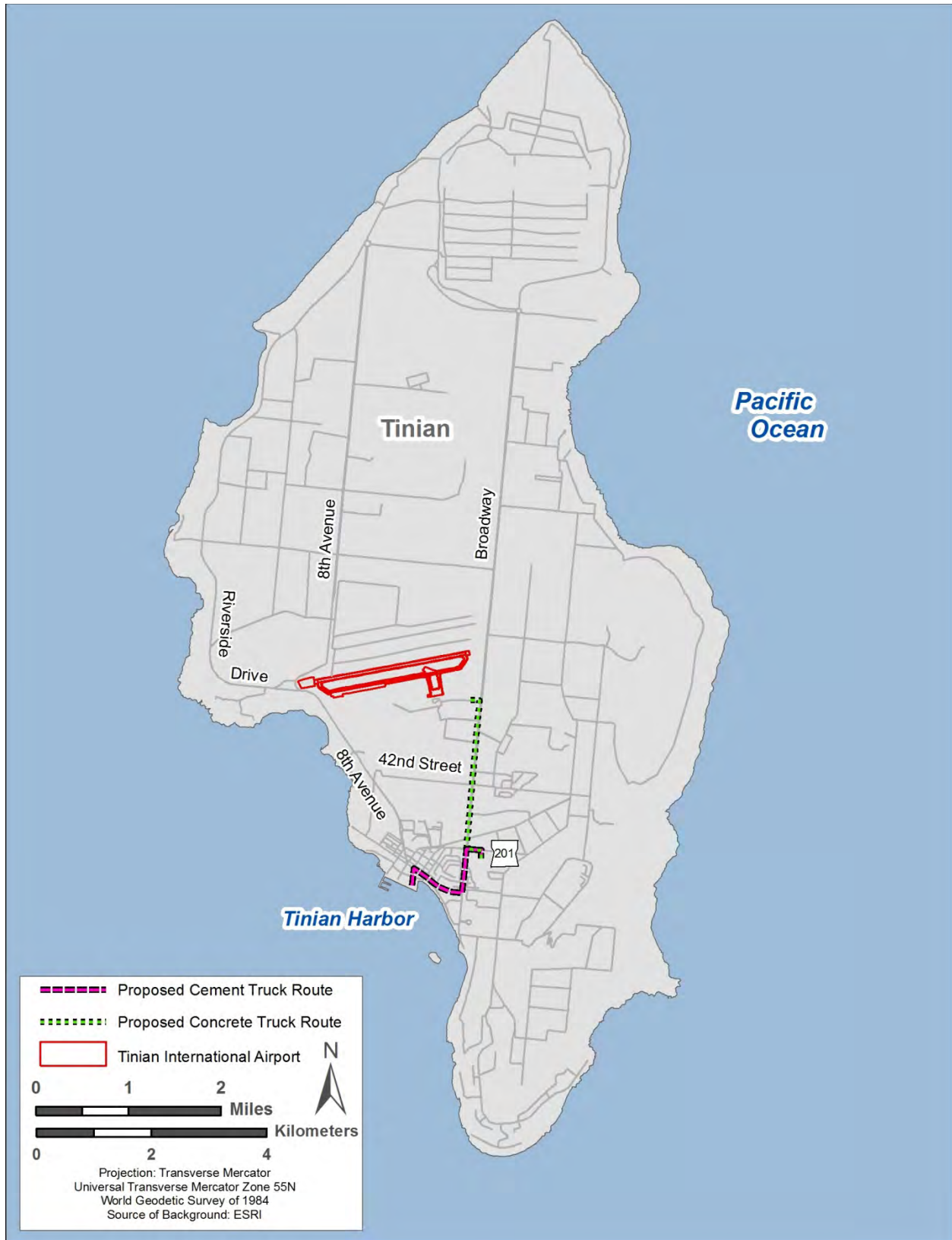
2 Figure 2.4-5. Proposed Cement and Concrete Truck Routes on Tinian
