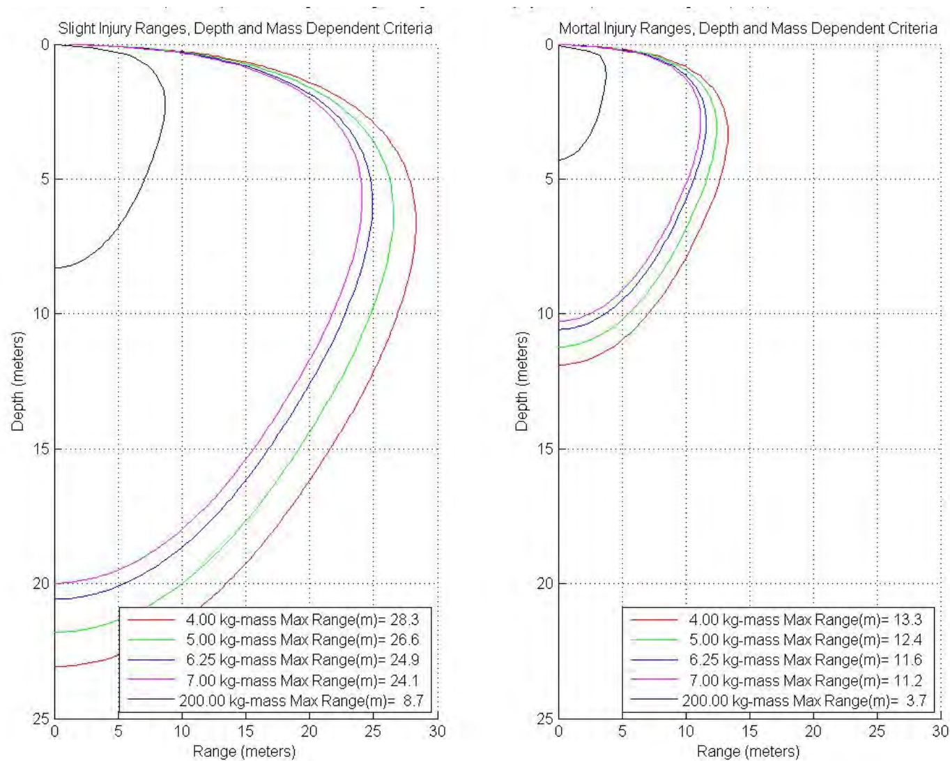
Figure 3.4-7: Threshold Profiles for Slight Lung Injury (left) and Mortality (right) Based on Five Representative Animal Masses for a 0.5-Pound Net Explosive Weight Charge (Bin E2) Detonated at 1-Meter Depth
